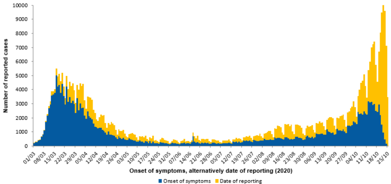
Figure 1: Number of COVID-19 cases in Germany electronically reported to the RKI by the date of symptoms onset or – if unknown – alternatively by date of reporting since 01/03/2020 (26/10/2020, 12:00 AM).
