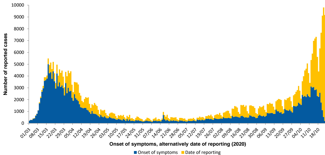
Figure 1: Number of COVID-19 cases in Germany electronically reported to the RKI by the date of symptoms onset or – if unknown – alternatively by date of reporting since 01/03/2020 (25/10/2020, 12:00 AM).
