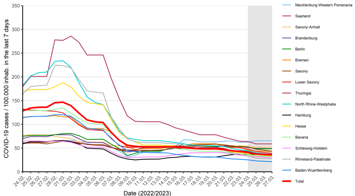
Figure 2: COVID-19 cases/100,000 inhabitants during 7 days in Germany by federal state and reporting date in the health offices (27/03/2023, 0:00 AM). The grey area delineates a range of dates with yet incomplete data, where changes in incidence are likely to occur.
