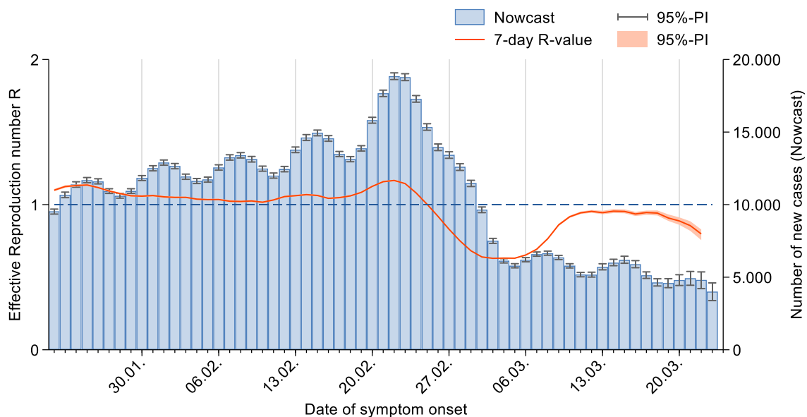
Figure 3: Estimated 7-day R-value (in orange) over the last 60 days, against the background of estimated number of COVID-19 cases according to illness onset (as of 27/03/2023, 12 AM, taking into account cases up to 23/03/2023).
