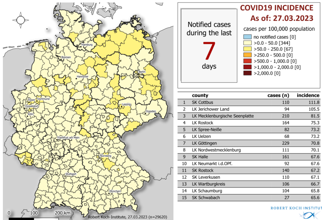
Figure 1: Number and cumulative incidence (per 100,000 population) of reported COVID-19 cases in Germany by county and federal state (n=29,620, 27/03/2023, 12:00 AM). Cases are usually reported according to the district from which they were transmitted. This usually corresponds to the place of residence. Place of residence and probable place of infection do not have to coincide.
