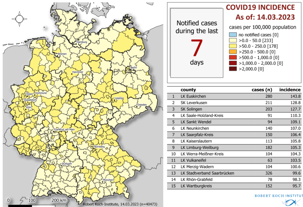
Figure 1: Number and cumulative incidence (per 100,000 population) of reported COVID-19 cases in Germany by county and federal state (n=40,473, 14/03/2023, 12:00 AM). Cases are usually reported according to the district from which they were transmitted. This usually corresponds to the place of residence. Place of residence and probable place of infection do not have to coincide.
