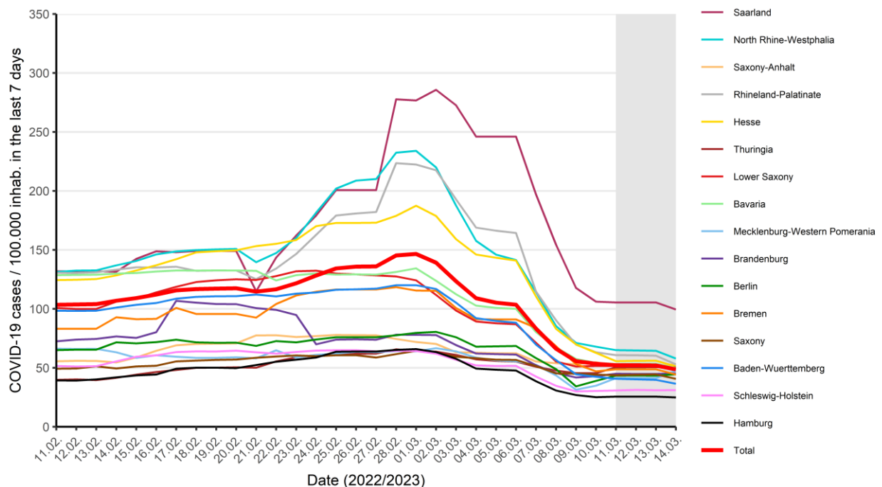
Figure 2: COVID-19 cases/100,000 inhabitants during 7 days in Germany by federal state and reporting date in the health offices (14/03/2023, 0:00 AM). The grey area delineates a range of dates with yet incomplete data, where changes in incidence are likely to occur.
