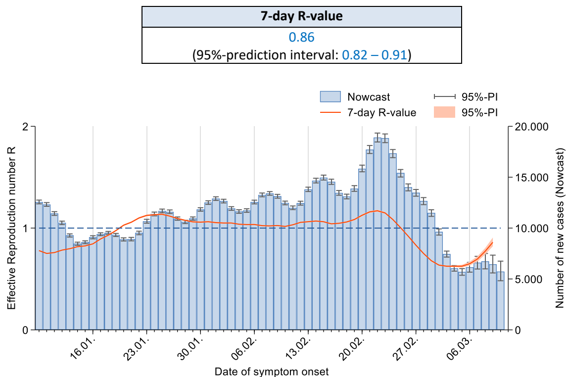
Figure 3: Estimated 7-day R-value (in orange) over the last 60 days, against the background of estimated number of COVID-19 cases according to illness onset (as of 14/03/2023, 12 AM, taking into account cases up to 10/03/2023).
