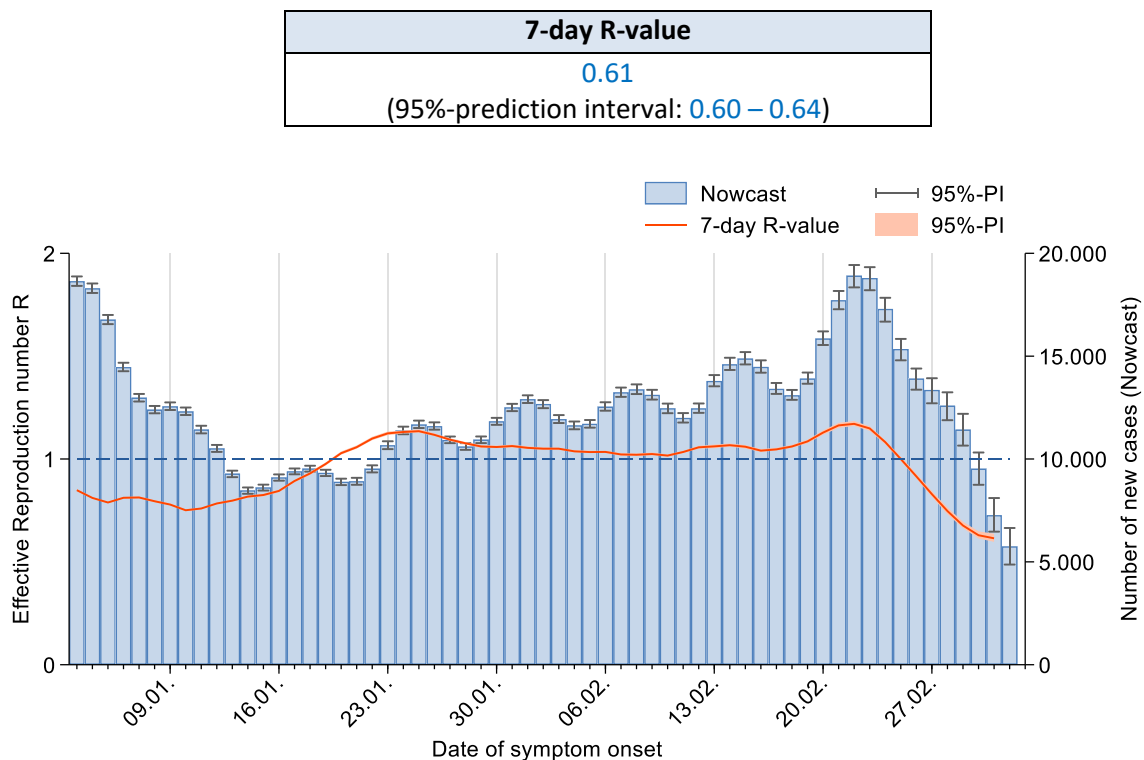
Figure 3: Estimated 7-day R-value (in orange) over the last 60 days, against the background of estimated number of COVID-19 cases according to illness onset (as of 08/03/2023, 12 AM, taking into account cases up to 04/03/2023).
