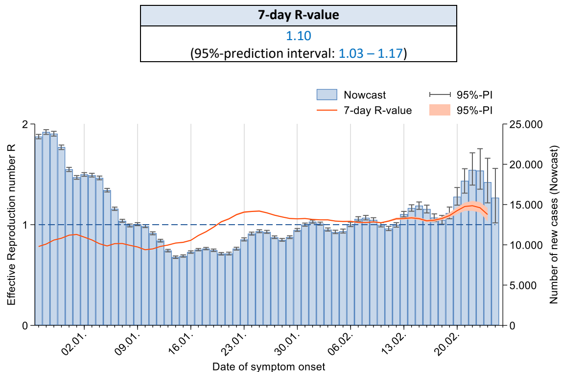
Figure 3: Estimated 7-day R-value (in orange) over the last 60 days, against the background of estimated number of COVID-19 cases according to illness onset (as of 01/03/2023, 12 AM, taking into account cases up to 25/02/2023).
